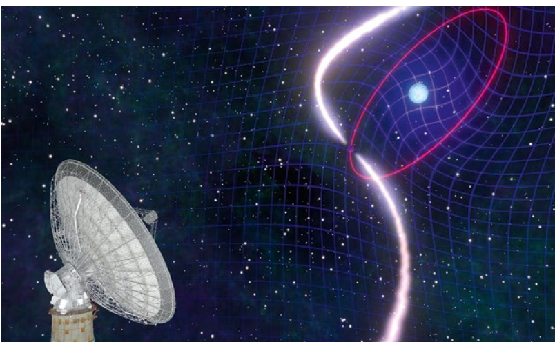
Mark Myers, OzGrav ARC Centre of Excellence
